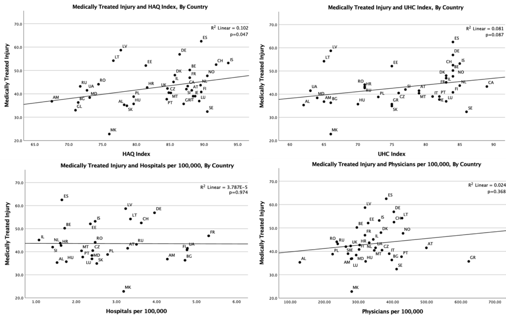
Supplementary Figure 2. Any medically treated injury and four country-level indicators of health services access: HAQ Index, UHC Index, Hospitals per 100,000, and Physicians per 100,000
